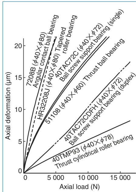
Fig. 1 Axial rigidity of various bearings
